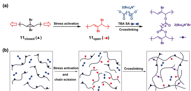
Fig. 12 (a) A gDCC mechanophore within a polymer chain under tension undergoes a ring-opening reaction from 11 closed to 11 open . This increases the contour length and provides an allylic bromide that is capable of self-strengthening through nucleophilic displacement reactions. (b) System-wide force causes chain scission, but also activates the mechanophore (black triangle to red dot), which subsequently reacts with a crosslinker (blue) to form an active crosslink (purple) that overcomes the damage. Reproduced with permission. 50 Copyright 2013, Springer Nature.
