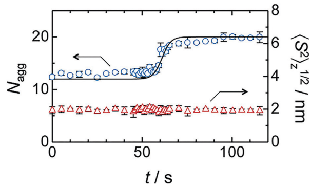
Fig. 5 Time evolution of N_{\text{agg}} (blue circles) and the radius of gyration \langle S^2 \rangle_z^{1/2} (red triangles). The solid curve for N_{\text{agg}} represents the fitted model curve. Reprinted with permission from ref. 133. Copyright 2017 from Wiley-VCH Verlag GmbH & Co. KGaA, Weinheim.
