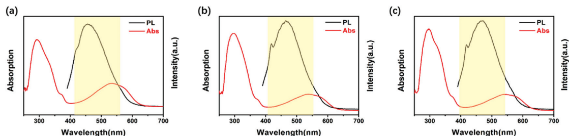
Fig. 4 UV-Vis spectra of closed ring forms (red line) and emission spectra of open ring forms (black line) of DTE6FPI (a), DTEHPMPI (b), and DTEODPI (c).
