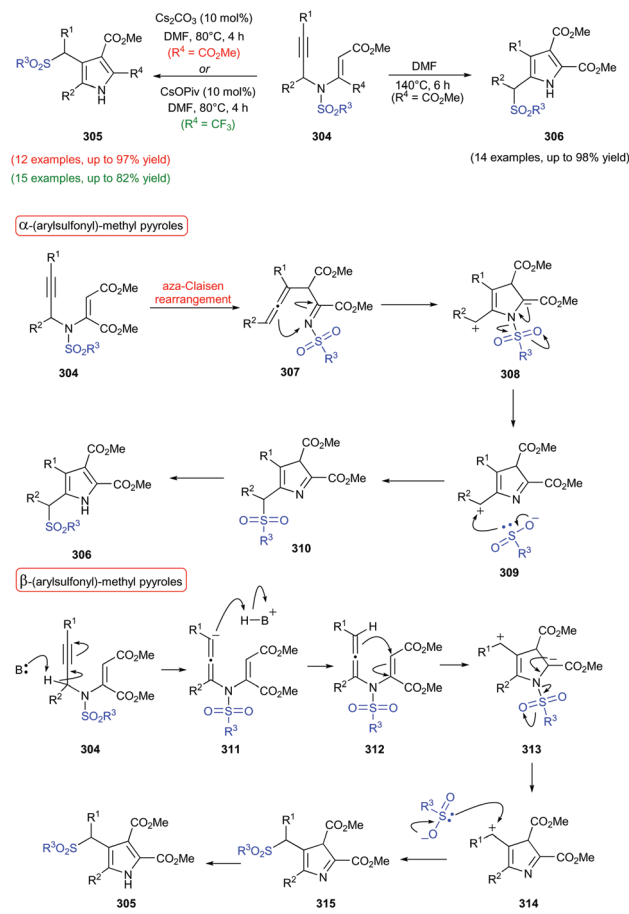
Scheme 43 Thermal aza-Claisen rearrangement of N -allyl ynamides and subsequent 1,3-sulfonyl migration.
