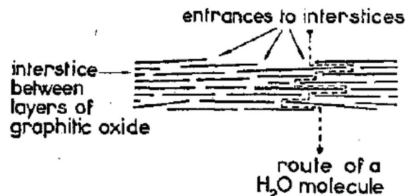
Fig. 4 Zigzag pathway of water permeation across the graphene oxide (graphite oxide) membrane. The size of permeation “channels” is provided by the distance between neighboring graphene oxide flakes and by the effect of swelling in water. 21
