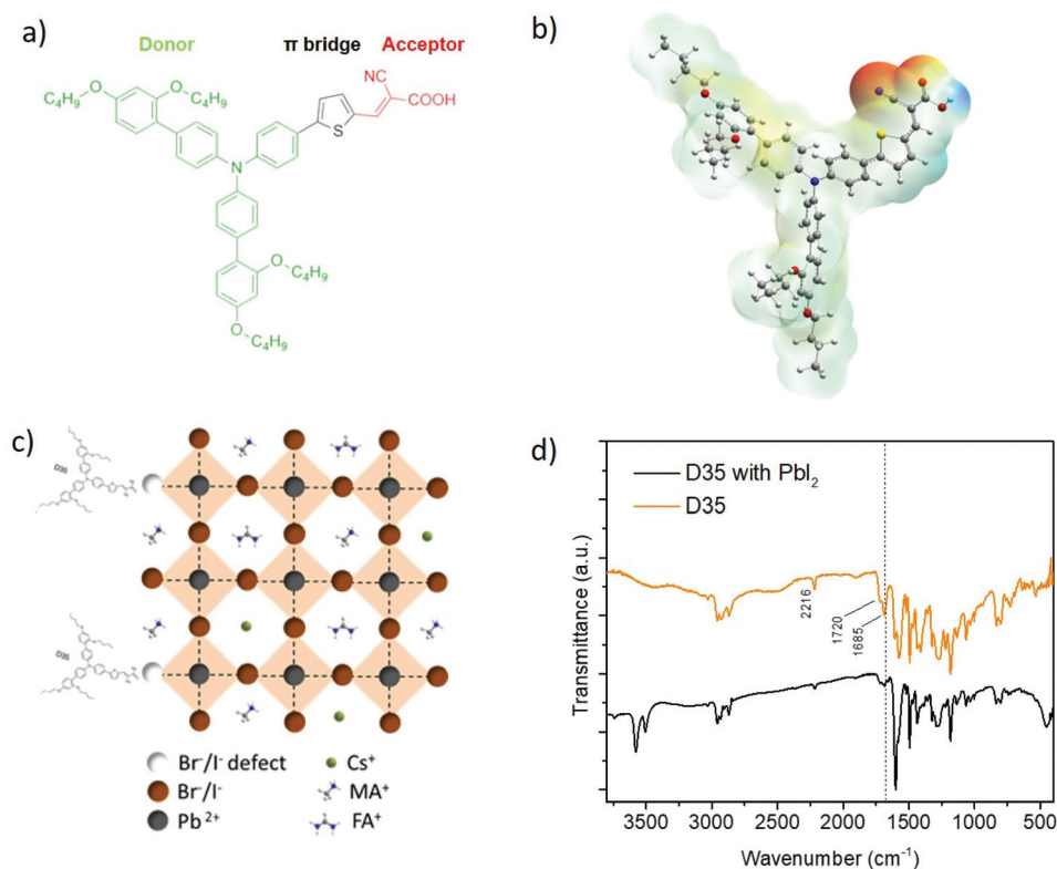
Fig. 1 Chemical structure of D35 (a); calculated ESP profiles of D35 (b); schematic illustration of the passivation process of D35 molecules for the under-coordinated Pb^{2+} cations (c); Fourier-transform infrared spectroscopy (FTIR) measurements in D35 with and without PbI_2 (d).
