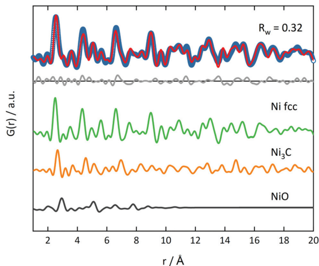
Fig. 8 PDF refinement of Ni(BDC)(PNO) decomposed at 375 °C in \text{H}_2 with three phases ( \text{Ni}_{\text{fcc}} , \text{Ni}_3\text{C} and \text{NiO} ). Blue open circles represent the experimental PDF and red line the calculated PDF. The grey line in the offset shows the difference between experimental and calculated PDF.
