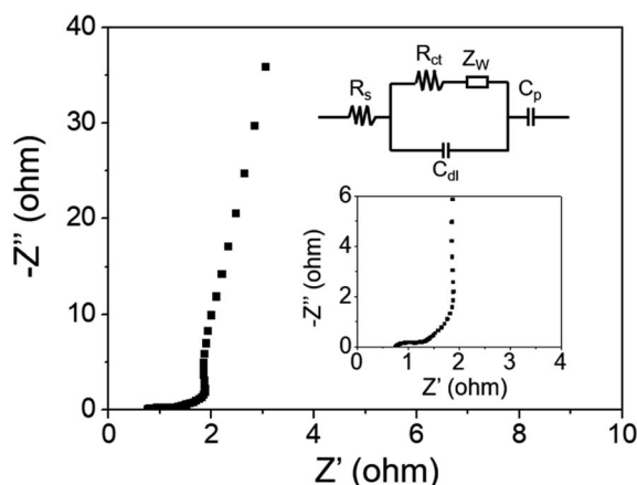
Fig. 10 Nyquist plot of the \text{MgCo}_2\text{O}_4 -NF-modified electrode and the inset is the enlarged plot in the high frequency region as well as the corresponding equivalent circuit.
