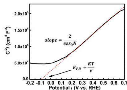
Fig. 7 Mott–Schottky plot for gel-derived UO 2 nanoparticles.
