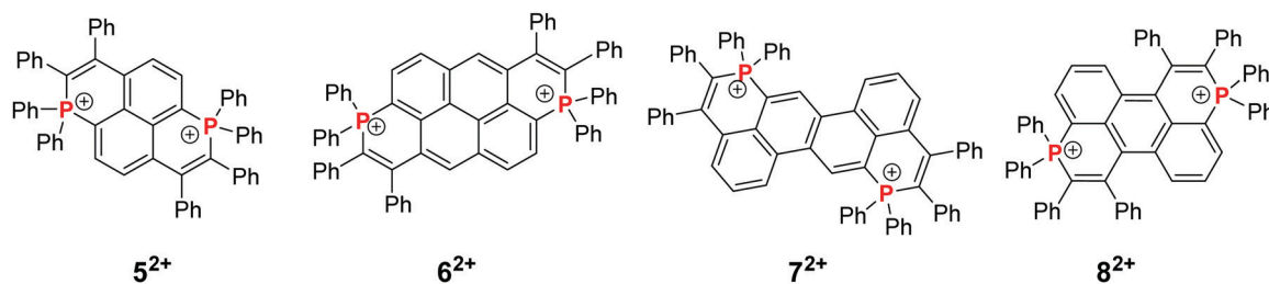
Fig. 2 Molecular structures of previously reported 5–8 2+ . 8
