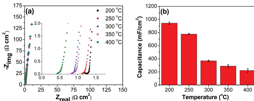
Fig. 10 (a) Nyquist plots for RuO 2 -CNF electrodes prepared at different temperatures (inset: the zoomed-in high-frequency region). The spectra were recorded at cell potential of 0 V (b) capacitance values obtained from EIS measurements for electrodes prepared at different temperatures.
