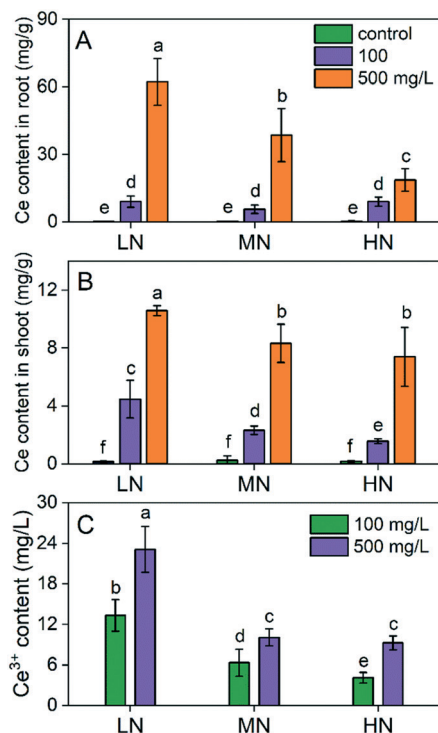
Fig. 7 Ce content in plant roots (A) and shoots (B) and the dissolution of \text{CeO}_2 NPs (C) in root exudates extracted under different N conditions. Different lowercase letters indicate significant difference at P < 0.05 .
