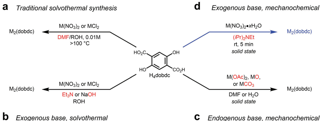
Fig. 2 Overview of methods for the synthesis of MOF-74 analogues, with the source of base highlighted in red. (a) Traditional solvothermal synthesis using N,N -dimethylformamide (DMF); (b) solvothermal synthesis using exogenous organic or inorganic base; (c) mechanochemical synthesis using basic metal precursors, and (d) mechanochemical synthesis using exogenous organic base (this work, highlighted in blue).
