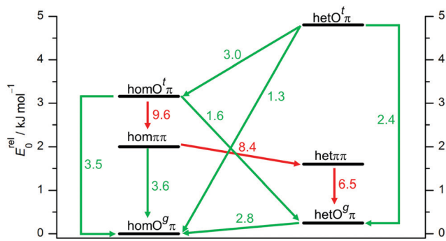
Fig. 4 Interconversion paths between B dimer structures including downhill barriers in \text{kJ mol}^{-1} at B3LYP-D3 level which are more (green) or less (red) feasible under supersonic jet expansion conditions. Transition structures are given in the ESI†
