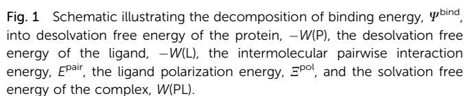
W_{\text{OBC2}}^{\text{bind,np}} differs from W_{\text{OBC2}}^{\text{bind}} because q_A^{\text{QM}} are used for ligand partial charges in the W(\text{PL}) calculation. \psi_{\text{OBC2}}^{\text{bind,np}} is the binding energy for a purely MM model.
