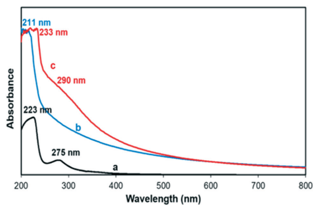
Fig. 9 UV-vis spectra of a) GA, b) ZIF-8, and c) ZIF-8-GA.
