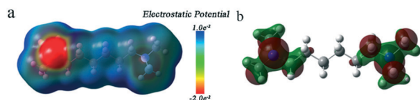
Fig. 5 (a) Molecular electrostatic potential map (MEP); (b) molecular orbital surfaces of N,N,N,N -tetramethyl-1,6-hexanediamine (white ball = hydrogen atom; gray ball = carbon atom; blue ball = nitrogen atom).
