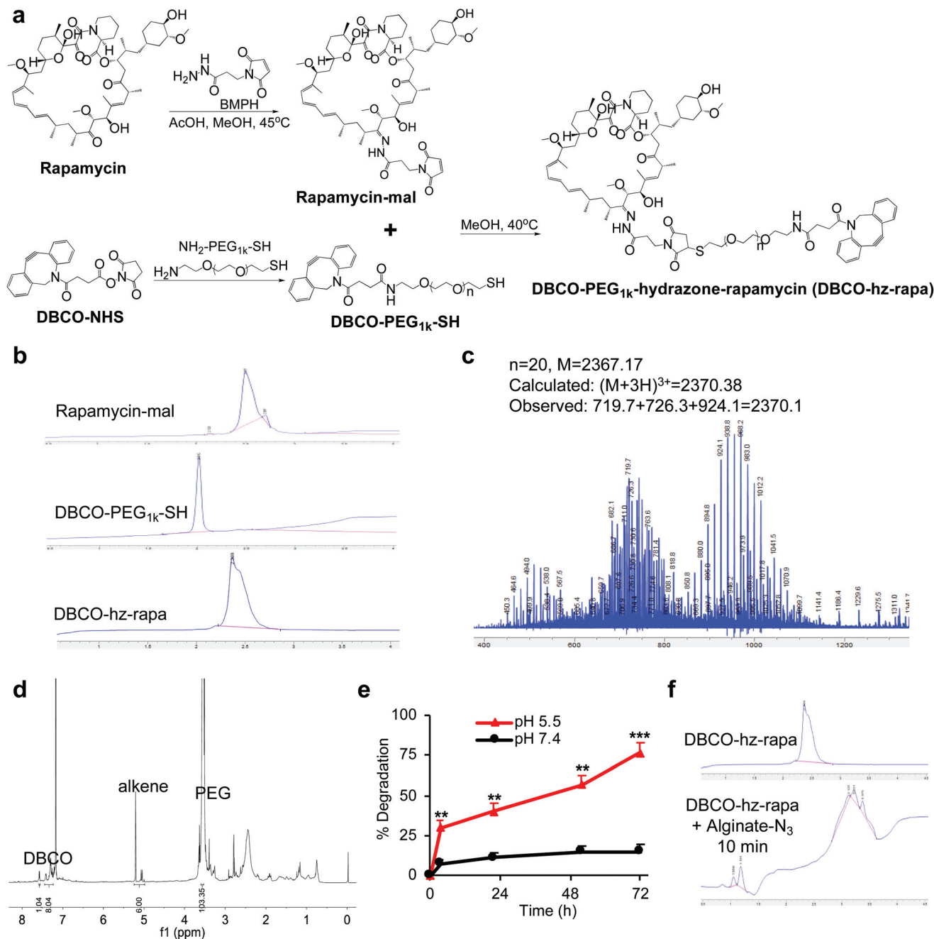
Fig. 1 Synthesis and characterizations of Clickable, acid labile DBCO-hz-rapa. (a) Synthetic route of DBCO-hz-rapa. (b) HPLC profiles of rapamycin-mal, DBCO-PEG 1k -SH, and DBCO-hz-rapa, respectively. (c) Mass spectrum of DBCO-hz-rapa. The interval of 14.7 ( m/z ) indicates the existence of [M + 3H]^{3+} . (d) 1 H NMR spectrum of DBCO-hz-rapa. (e) pH-Dependent degradation profiles of DBCO-hz-rapa to rapamycin under pH 7.4 and 5.5, respectively. Data were presented as mean \pm SD ( n = 4 ), and analyzed by two-tailed t -test ( 0.01 < *P \leq 0.05 ; **P \leq 0.01 ; ***P \leq 0.001 ). (f) HPLC traces of the mixture of DBCO-hz-rapa and alginate-N 3 , which showed rapid conjugation via Click chemistry.
