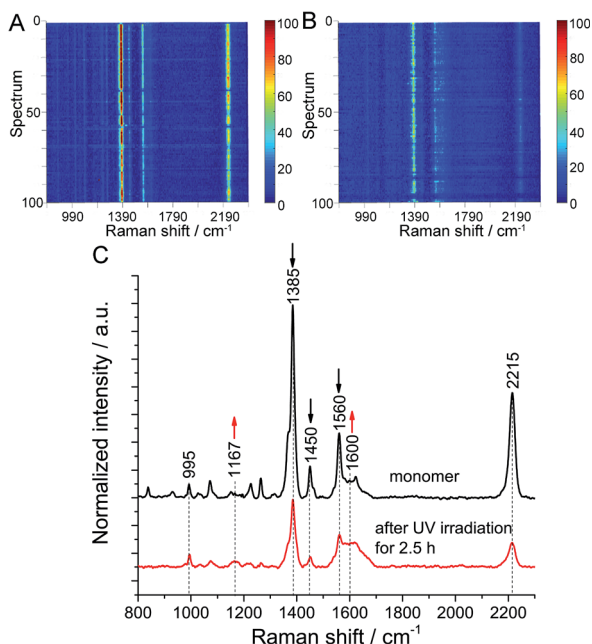
Fig. 3 Waterfall plot of all TERS spectra from maps of a monomer monolayer on Au (111) before (A) and after UV irradiation for 2.5 h (B). The size of all maps is 1 × 1 μm² with a 100 nm pixel size. (C) Baseline corrected average TER spectra from the above two TERS maps. These two TER spectra were normalized to the Raman peak at 995 cm -1 .
