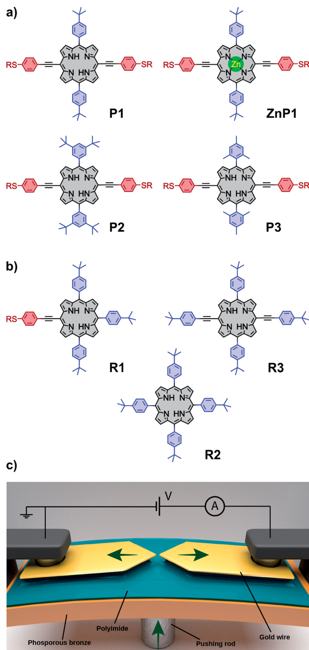
Fig. 1 (a) Structural designs of P1 , ZnP1 , P2 and P3 ; (b) structural formulae of R1 , R2 and R3 . The different parts of the molecule have been coloured dividing the anchoring groups (red) and the bulky side groups (blue). The molecules are synthesized with R = acetyl, but upon deprotection at the electrode surface, R represents either a hydrogen atom or the gold electrode. (c) Schematics of the mechanically controllable break-junction (MCBJ) setup.
