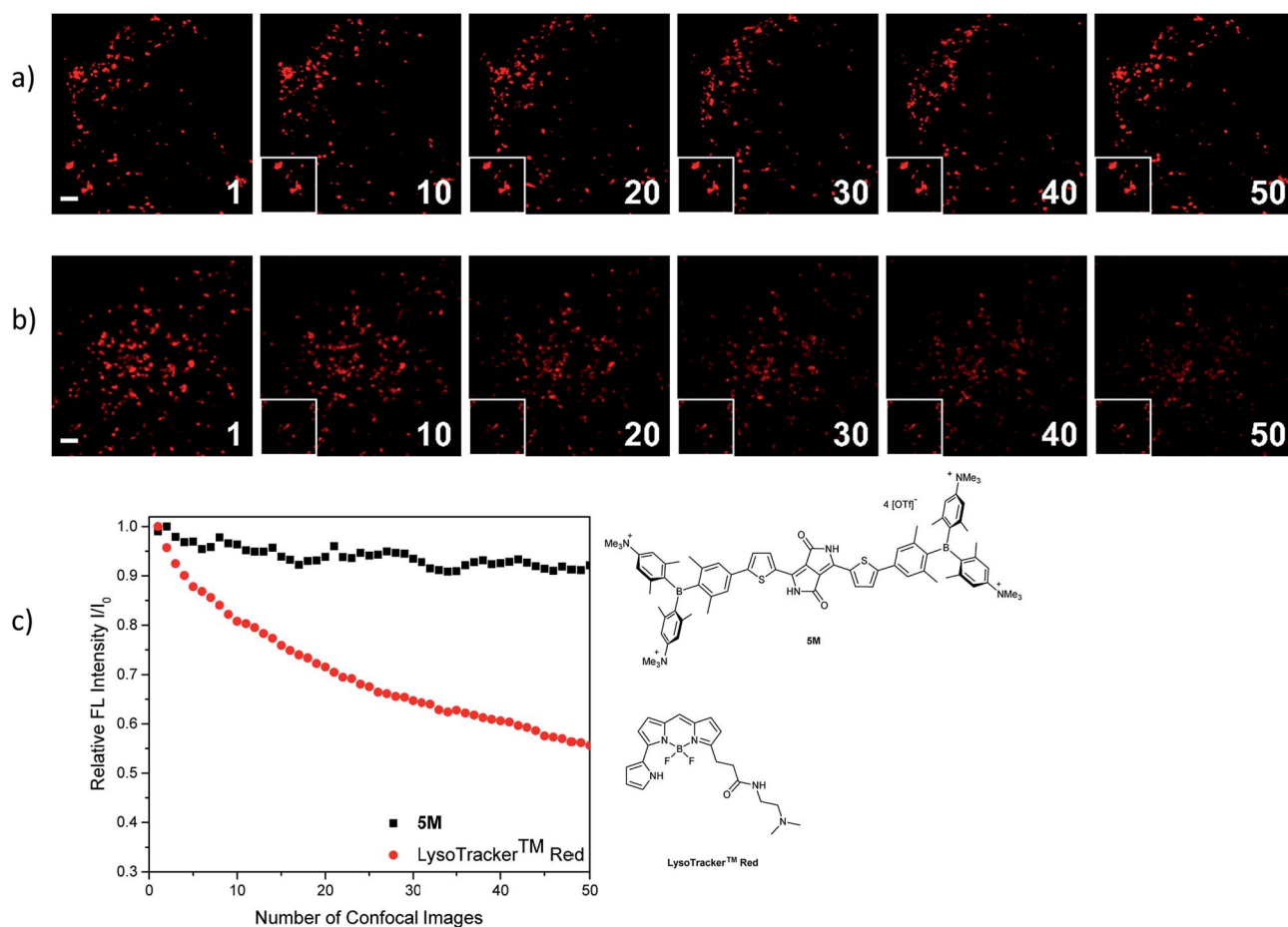
Fig. 11 Comparison of the repeated fluorescence images of HeLa cells stained with (a) 5M and (b) LysoTracker TM Red under irradiation with a confocal laser at 561 nm (WLL, output power 70%, AOTF 2%). Each number indicates the number of recorded confocal images. The rectangle (bottom, left in each picture) is the cutout of the image at n = 1 . Scale bar: 2 \mu\text{m} . (c) Plots of integrated fluorescence intensities ( I ) relative to the initial value ( I_0 ) as a function of the number of recorded images.
