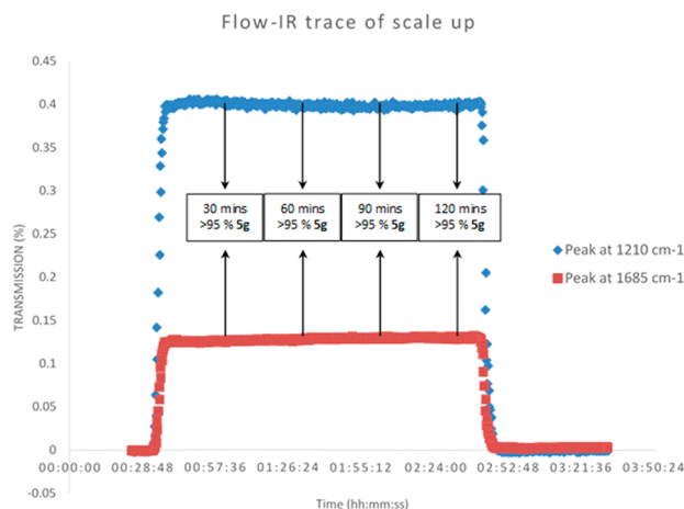
Fig. 5 Flow scale-up of 5-Br isoquinoline 3a and N -Boc pyrrolidine. Under optimized conditions, a flow rate of 1 \text{ mmol min}^{-1} ( \tau = 10 \text{ min} ) was achieved. Using inline IR monitoring, the process was shown to be stable and can be operated at the steady state for prolonged periods, demonstrating the feasibility of the process for multi-gram production.
