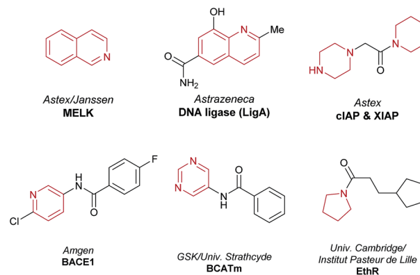
Fig. 6 Fragment hits used as starting points for F2L campaigns reported in 2015 and 2016. All contain heterocycles within the reactivity scope of the \text{C}(\text{sp}^2)\text{--C}(\text{sp}^3) cross-dehydrogenative coupling reported herein.
