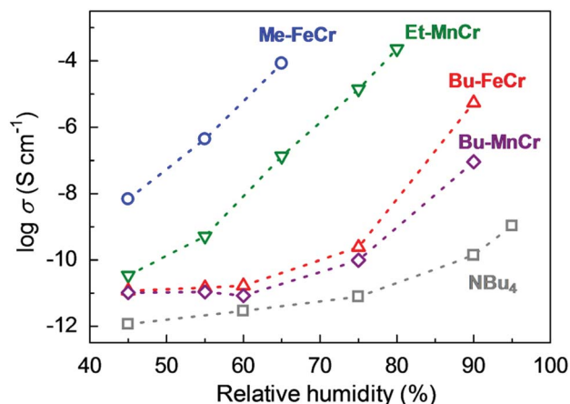
Fig. 6 Humidity dependence of the proton conductivity at 298 K. The blue, green, red, purple, and gray colors correspond to the proton conductivity of Me-FeCr, Et-MnCr, Bu-FeCr, Bu-MnCr, and \text{NBu}_4 , respectively. Reproduced from ref. 49 with permission from American Chemical Society, Copyright 2012.
