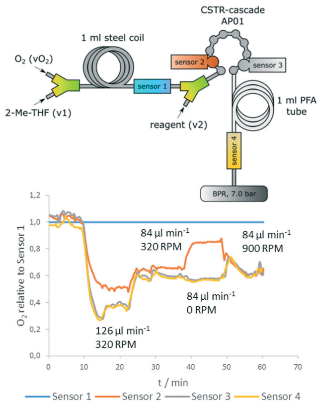
Fig. 10 Flow setup with sensor arrangement in the reactor (top); relative oxygen content in the reactor at varying reagent flow rate v_2 (1 M 4-methoxyphenylmagnesium bromide). v_{O_2} : 1500 \mu\text{l min}^{-1} , v_1 : 1000 \mu\text{l min}^{-1} (bottom).
