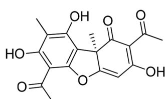
(-)-Usnic acid
