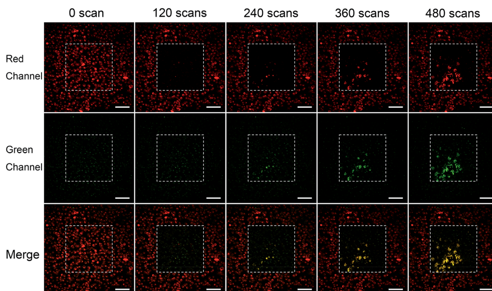
Fig. 5 Evaluation of localized PDT after treated with BT-RB nanoparticles under 1040 nm fs laser irradiation. The white dashed lines square out the scanning areas. Scale bar: 100 \mu\text{m} .
