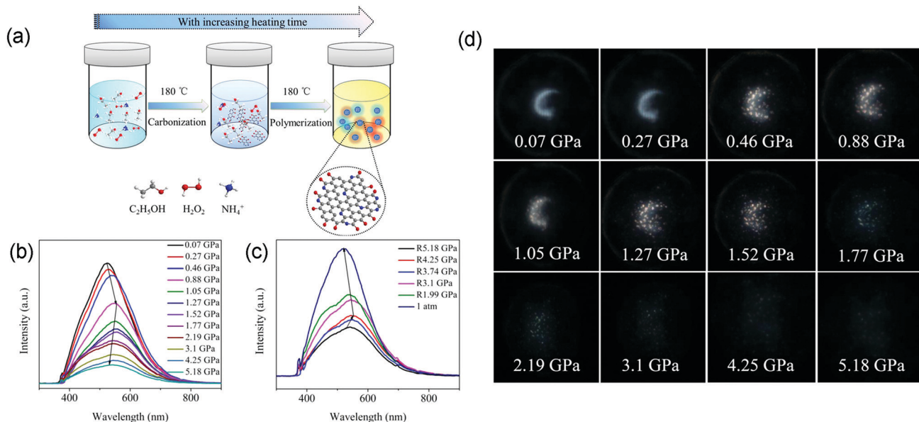
Fig. 5 (a) Schematic of the facile synthesis of N-CDs via a one-step ethanol-thermal strategy treated with H_2O_2 and NH_3-H_2O . (b) PL spectra of N-CDs with increasing pressure. (c) PL spectra of N-CDs as the pressure decreases to ambient conditions. (d) Optical photographs of N-CDs with increasing pressure. Reproduced with permission from ref. 43. Copyright 2018 American Chemical Society.
