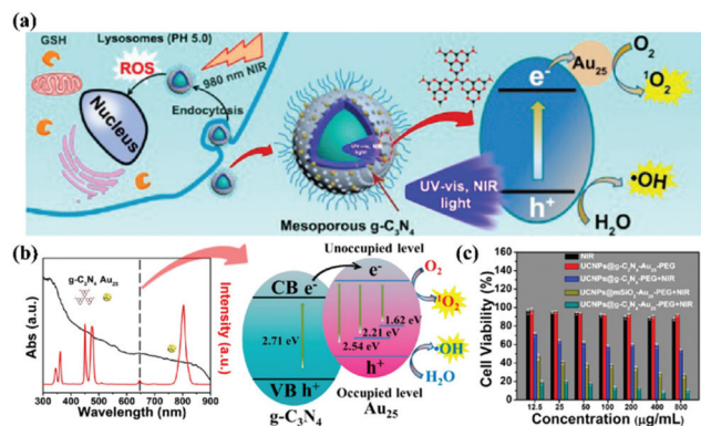
Fig. 7 Improving the excitation light conditions of g-CNs optimizes PDT. (a) g-CNs combined with UCNPs changes the excitation source to near-infrared light and can be combined with the Jinnai cluster to improve the effect of PDT. (b) g-CNs and Au 25 have overlapped absorption and luminescence, both of which effectively absorb the light emitted by UCNPs. The difference in the energy levels between g-CNs and Au 25 can expand the transition of electrons, convert O 2 to O 2 - and convert H 2 O to OH - . (c) When g-CNs are combined with Au 25 , the photodynamic effect is significantly improved. Significant differences can be obtained through biotoxicity testing. Reproduced with permission. 67 Copyright 2017, American Chemical Society.
