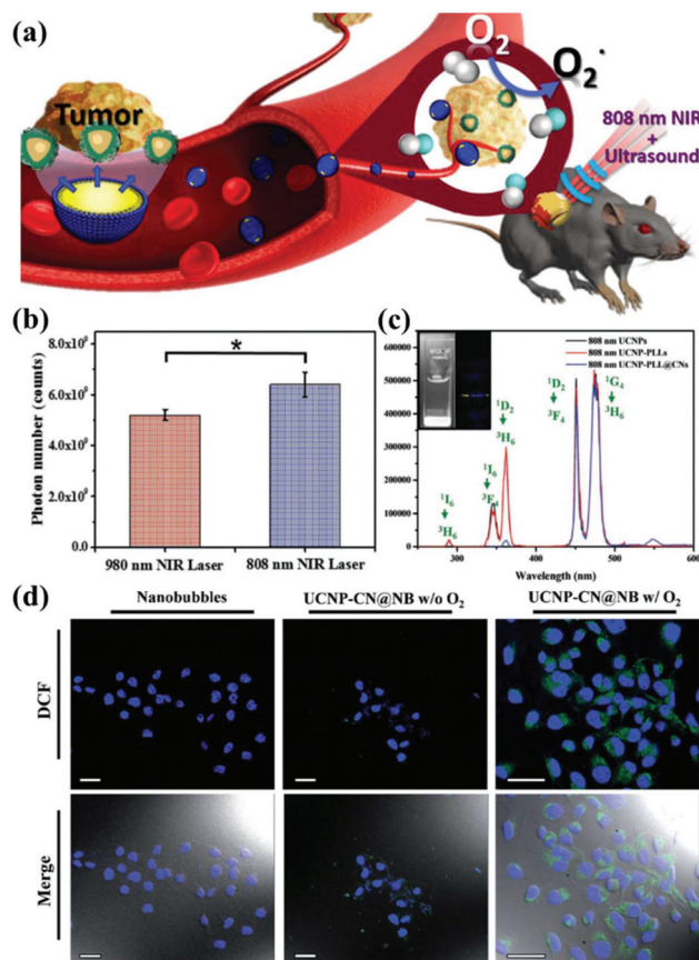
Fig. 8 g-CN-based biotherapy with UCNPs. (a) g-CNs combined with 808 nm-excited UCNPs and nanobubbles to form advanced theranostic nanoplatforms. (b) Photon quantification of UCNPs@CN bio-luminescence images with 980 nm and 808 nm NIR irradiation. (c) Photoluminescence spectra of 808 nm-excited UCNPs-PLL@Cns (inset: the digital fluorescence photographs of nanocomposites have both blue and green fluorescence). Reproduced with permission. 70 Copyright 2017, Wiley Online Library. (d) Tumor cells treated with UCNPs-CN@NBs (500 μg mL -1 ) are exposed to an 808 nm laser. The cells were stained with DCF detection dye. An increase in green fluorescence in irradiated cells indicates ROS production. Reproduced with permission. 71 Copyright 2018, Royal Society of Chemistry.
