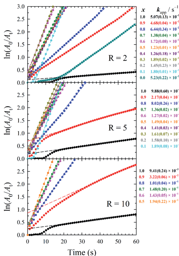
Fig. 3 Plots depicting the pseudo-first-order kinetics of 4-NP reduction and associated catalytic rates ( k_{\text{app}} ) using 5 d-old borohydride-stabilized \text{Au}_x\text{Ag}_{1-x} -NP nanocatalysts ( R = 2, 5 , and 10 , top to bottom). Excluded x values for a particular R value indicate the observation of appreciable colloidal precipitation after aging for 5 d.
