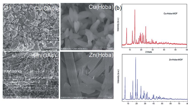
Fig. 1 (a) SEM images of MA precursors (left column) and their respective reaction products with Hobia in water and DMF. (b) PXRD patterns of the products synthesized in one minute.
