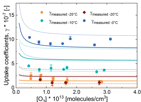
Fig. 6 Measured and parameterized uptake coefficients ( H_{O_3, \text{Mix\_CAsalt-in(T-ind)}} ) with error bands at different temperatures as a function of gas-phase ozone concentration. The dots are the measured uptake coefficients; the solid lines are the model lines; the thin dashed lines are the error bands for the parameterization output. The parameterization output and error bands have the same colour as the temperature in question: blue circles for 0 °C, cyan pentagons for −10 °C, red diamonds for −20 °C, and orange squares for −25 °C.
