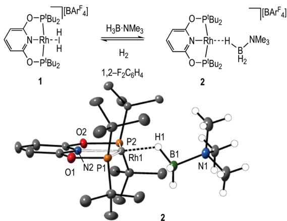
Fig. 1 Synthesis and solid-state structure of complex 2. Displacement ellipsoids shown at the 30% level. [BARF 4 ] − anion and most H-atoms are not shown for clarity. Selected bond distances (Å) and angles (°): Rh1–B1, 2.567(5); Rh1–P1, 2.2832(9); Rh1–P2, 2.2594(9); Rh1–N2, 2.026(3); B1–N1, 1.631(6); Rh1–H1, 1.72(5); P1–Rh1–P2, 161.63(3); N2–Rh1–H1, 172.6(17); Rh1–H1–B1, 121(4).
