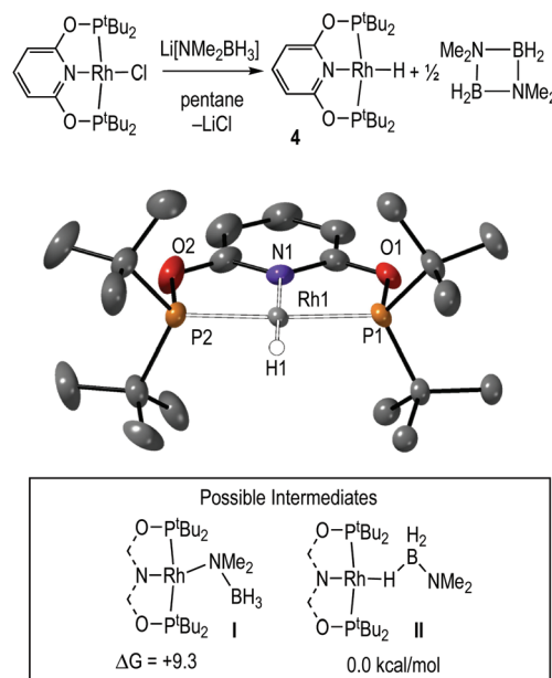
Fig. 3 Independent synthesis, solid-state structure of complex 4, and possible intermediates. Displacement ellipsoids shown at the 30% level. Most H-atoms are not shown for clarity. Selected bond distances (Å) and angles (°): Rh1-H1, 1.54(5); Rh1-P1, 2.2179(17); Rh1-P2, 2.2020(17); Rh1-N1, 2.046(6); P1-Rh1-P2, 162.80(7). Free energies are DFT-calculated.
