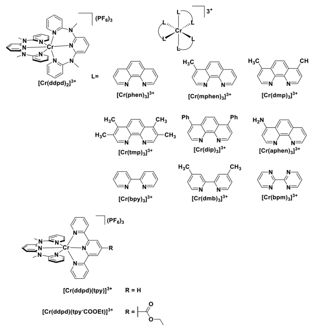
Fig. 34 Chromium(III) complexes.
