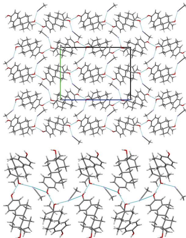
Fig. 4 (top) Packing diagram of BES-ACN, viewed down the a axis. (bottom) Hydrogen bonding between the estradiol hydroxyl groups and acetonitrile molecules (c.f. Chain 2 ESI † Fig. S17). Light blue lines indicate hydrogen bonding.
