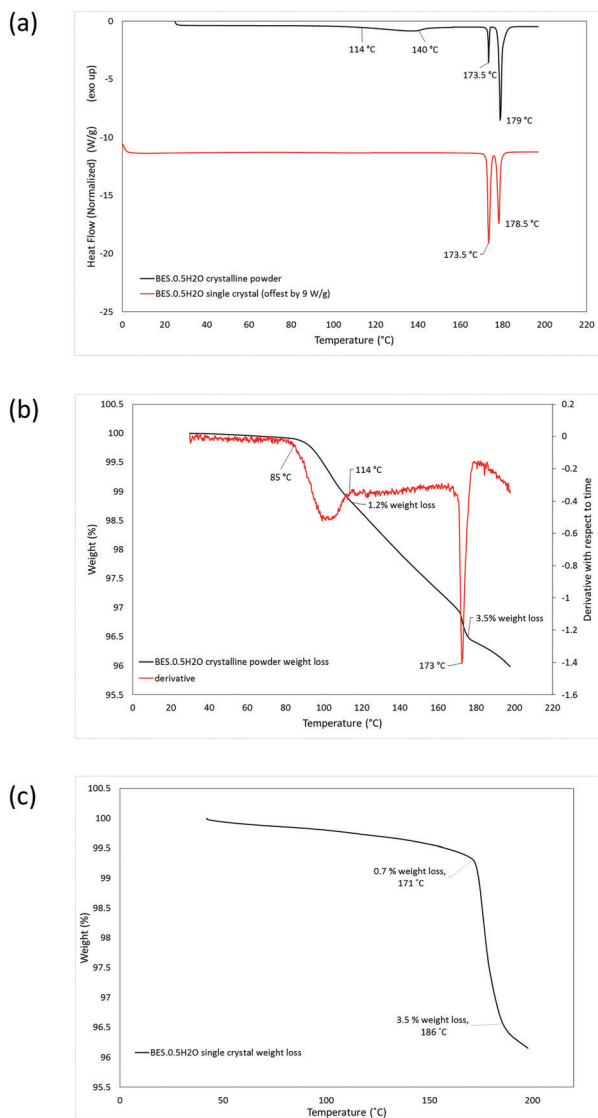
Fig. 5 DSC and TGA traces of BES.0.5H 2 O. (a) DSC curve of a crystalline powder (black) and a single crystal (red). (b) TGA curve of a crystalline powder (black) including derivative with respect to time (red). (c) TGA curve of a single crystal form.
