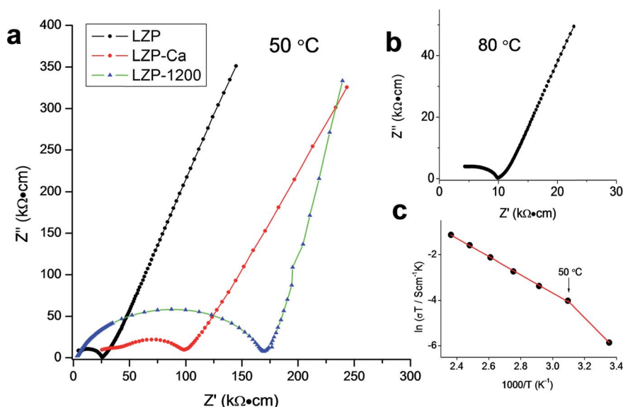
Fig. 3 (a) Typical impedance plots of LZP-1100, LZP-Ca and LZP-1200 at 50 °C using Au electrodes. (b) Impedance plot for LZP-1100 at 80 °C using Au electrodes. (c) Arrhenius plot for the total conductivity of LZP-1100 in the temperature range 25–150 °C.
