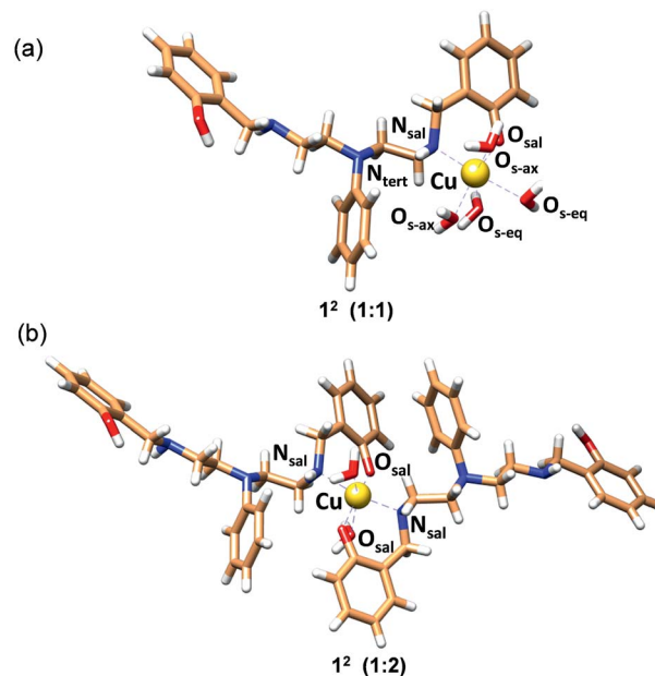
Fig. 3 MOMEc optimized structures for (a) [\text{Cu}^{2+}(\text{2c})(\text{OH}_2)_4] ( 1^2 ; 1 : 1) and (b) [\text{Cu}^{2+}(\text{2c})_2(\text{OH}_2)_2] ( 1^2 ; 1 : 2) complexes. Ligand 2c is in the phenolate form. In the structures, carbon, nitrogen, oxygen and hydrogen atoms are represented in light brown, blue, red and white colors, respectively. Copper ions are represented in gold.
