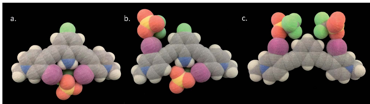
Fig. 8 3D prints generated from the crystal structures (vdW radii) of disordered G2XBme 2+ ·2OTf - the bidentate (a) and S conformations (b) and G1XBme 2+ ·2OTf - in the W conformation (c).
