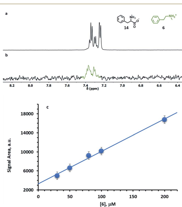
Fig. 9 (a) ^1\text{H} -NMR subspectrum of phenylalanine ( 14 , 1 mM) and N -methylphenethylamine ( 6 , 50 \mu\text{M} ). (b) STD subspectrum of the same mixture in the presence of S4 -AuNP (1024 scans, 3 h). (c) Plot of the integrated signal area of the aromatic signals of 6 in the STD spectra vs. [ 6 ]; the blue line represents the linear fit of the data ( R = 0.995 ). Conditions: [ S4 -AuNP] = 15 \mu\text{M} , HEPES buffer 10 mM, and pD = 7.0. The errors in the integral data (800 a.u.) were estimated by repeated integrations of the most intense signal at 200 \mu\text{M} and considered constant.
