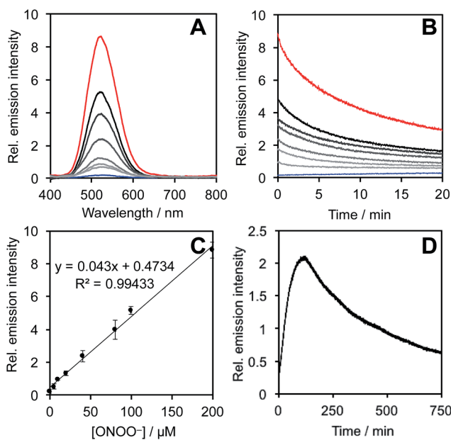
Fig. 1 Response of PNCL to \text{ONOO}^- . (A) Chemiluminescent emission spectra of 20 \mu\text{M} PNCL and 0 (blue trace), 5, 10, 20, 40, 80, 100, 200 \mu\text{M} (red trace) \text{ONOO}^- . (B) Time scans of the chemiluminescent emission at 525 nm of 20 \mu\text{M} PNCL and 0 (blue trace), 5, 10, 20, 40, 80, 100, 200 \mu\text{M} (red trace) \text{ONOO}^- . (C) Peak emission intensity at 525 nm of 20 \mu\text{M} PNCL after adding 0–200 \mu\text{M} \text{ONOO}^- . (D) Time scan of the chemiluminescent emission at 525 nm of 20 \mu\text{M} PNCL and 200 \mu\text{M} SIN-1. All experiments were performed in 20 mM HEPES (pH 7.4), containing <1% DMSO.
