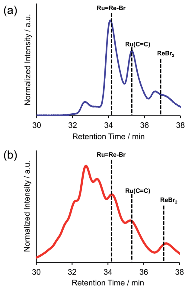
Fig. 1 Size-exclusion chromatogram measured after the reaction to obtain Ru=Re-Br (a) using \text{PPh}_3 and subsequent air injection and (b) in the absence of \text{PPh}_3 .
