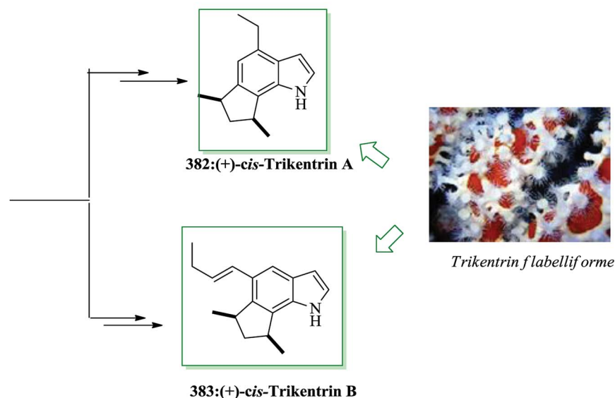
Scheme 81 Total synthesis of (+)-cis-trikentrin 382 and (+)-cis-trikentrin-B 383.
