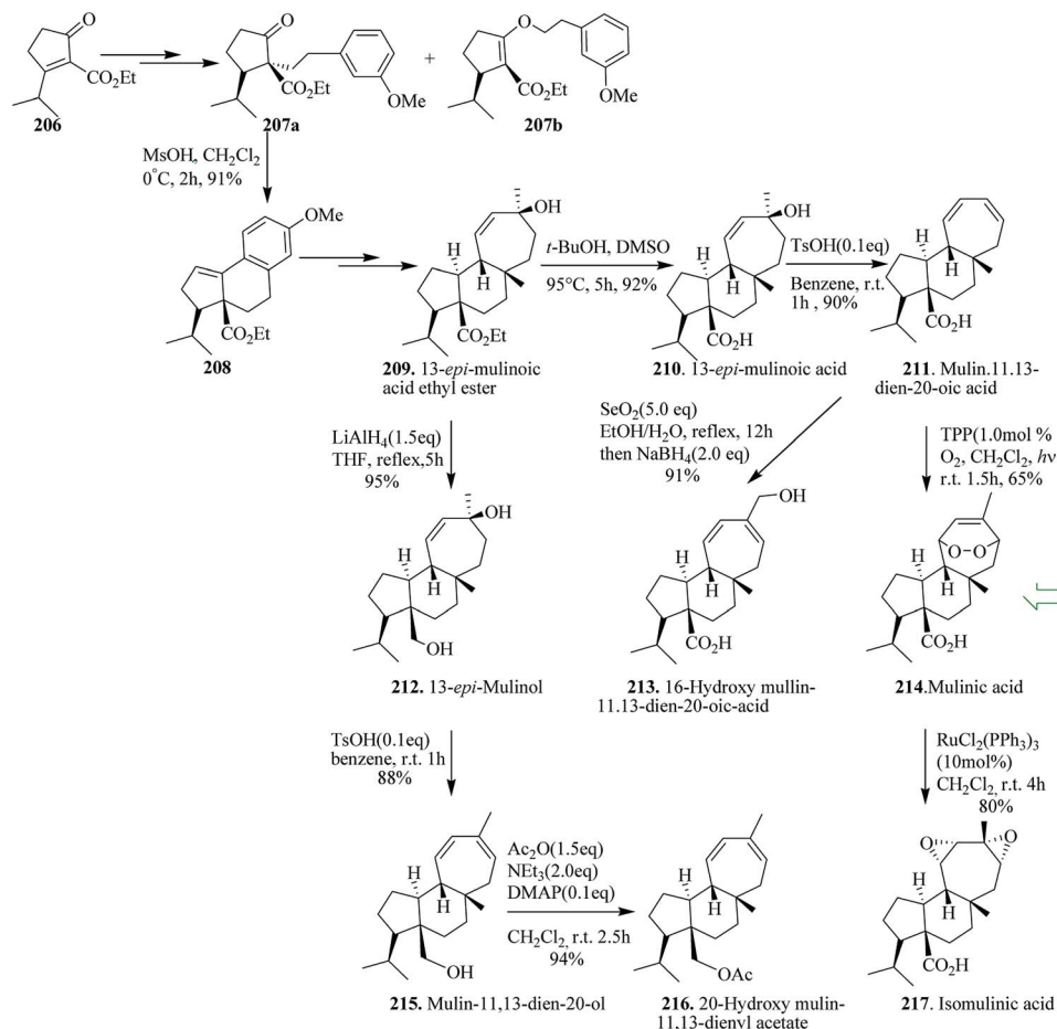
Scheme 45 Total synthesis of 13- epi -mulinolic acid ethyl ester 209 , 13- epi -mulinolic acid 210 , mulin-11,13-dien-20-oic acid 211 , 13- epi -mulinol 212 , 16-hydroxymulin-11,13-dien-20-oic acid 213 , mulinic acid 214 , mulin-11,13-dien-20-ol 215 , 20-hydroxy mulin-11,13-dienyl acetate 216 and isomulinic acid 217 .
