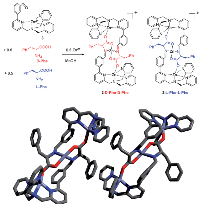
Fig. 4 X-ray crystal structure of 2-Phe starting from the racemic Phe. Both 2-D-Phe-D-Phe and the 2-L-Phe-L-Phe are present in the same unit cell. The counteranions are perchlorates.
