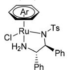
( S,S )- 1a : Ar = p -cymene ( S,S )- 1b : Ar = mesitylene
