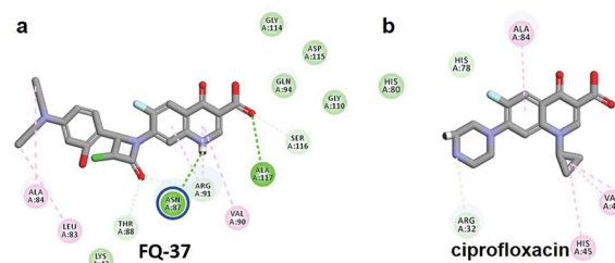
Fig. 8 (a) Hydrogen bond interaction of unsubstituted \text{-NH} group in molecule FQ-37 with mutant residue Asn87 (b) interactions of substituted \text{-NH} group in ciprofloxacin.
