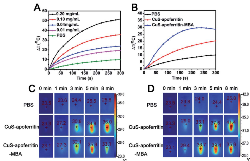
Fig. 4 The photothermal effect of (A) CuS-afoperritin and (B) CuS-afoperritin-MBA aqueous solutions irradiated by 808 nm laser light ( 0.8 \text{ W cm}^{-2} ). The infrared thermal images of CuS-afoperritin and CuS-afoperritin-MBA aqueous solution after 808 nm laser light irradiated for different times (1, 3, 5, and 8 min) at different concentrations (C) 100 \mu\text{g mL}^{-1} and (D) 200 \mu\text{g mL}^{-1} .
