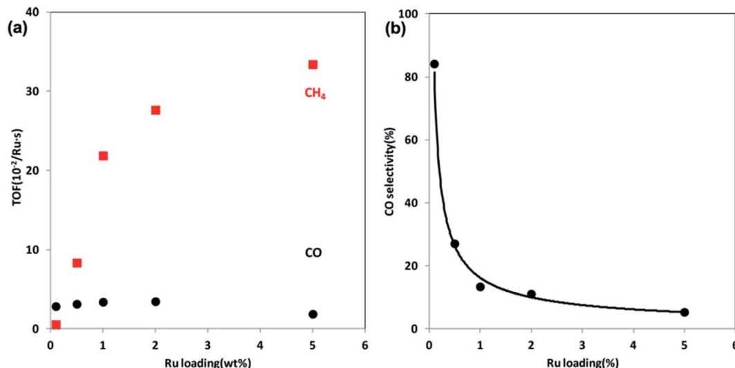
Fig. 6 (a) TOFs of \text{CO} and \text{CH}_4 formation at steady state at 300^\circ\text{C} over \text{Ru}/\text{Al}_2\text{O}_3 catalysts as a function of Ru loading. (b) \text{CO} selectivity as a function of Ru loading at 300^\circ\text{C} . Reprinted with permission from ref. 47. Copyright 2013 ACS.
