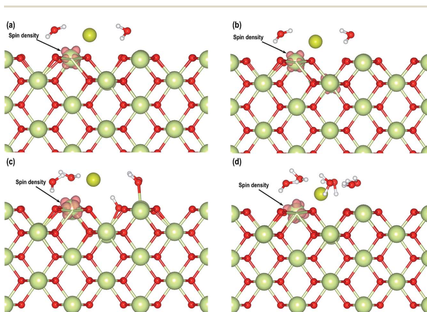
Fig. 10 (a) Electron spin density for model with two water molecules obtained by DFT+ U calculations at an isosurface of 0.007 e Å -3 . Electron spin density for model with (b) two, (c) four and (d) six water molecules obtained by DFT+ U +D3 calculations at an isosurface of 0.007 e Å -3 .
