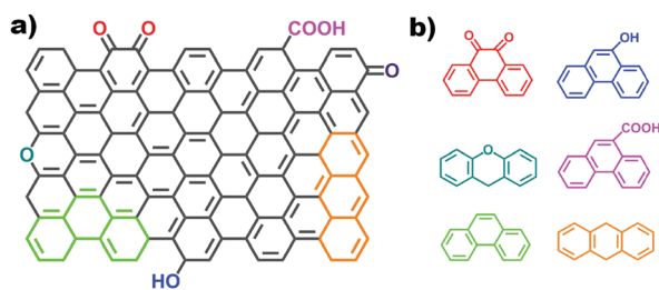
Fig. 11 (a) Surface structure of carbon materials with typical oxygen species and edge defects. (b) Structures of different aromatic organic molecules with single oxygen groups ( e.g. , C=O, C-OH, C-O-C, -COOH) and designed defect configurations ( e.g. , armchair and zigzag).
