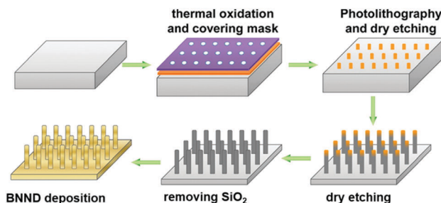
Fig. 13 Preparation of BNND/Si rod arrays, reproduced from ref. 180 with permission from American Chemical Society, copyright 2013.
