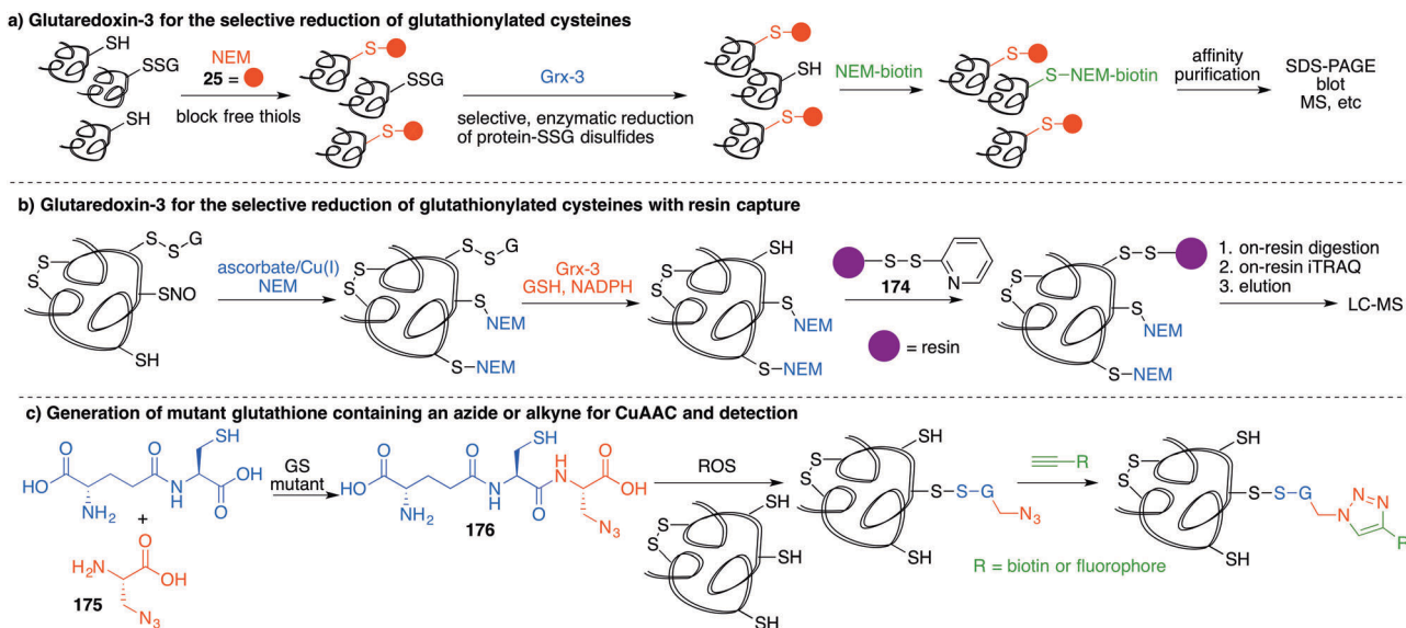
Fig. 23 (a and b) Glutaredoxin-3 (Grx-3) can selectively reduce protein-S-SG disulfides. After blocking free thiols, Grx-3 can be used to reduce the sites of glutathionylation. The resulting cysteine thiols can then be labelled for affinity enrichment and further analysis. In (b), a resin-capture ( 174 ) is used to improve detection of reduced glutathione thiols. (c) Glutathione containing an azide or alkyne ( 176 ) incorporated using a mutant GS can react with reactive thiols and later be detected by using an alkyne or azide with a reporter group for analysis.
