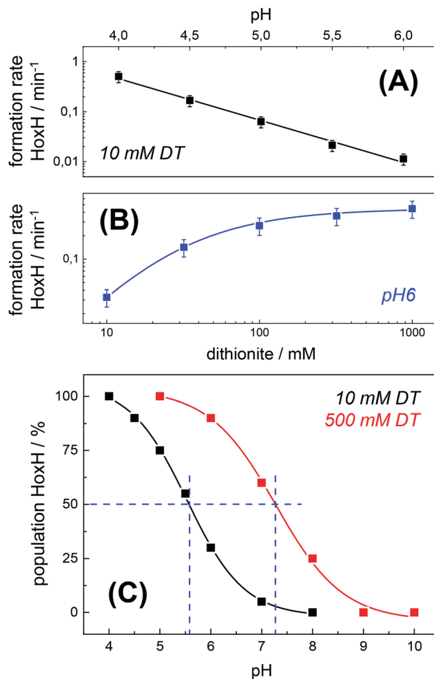
Fig. 5 Rate and yield of Hox \rightarrow HoxH conversion in \text{HYDA1}^{\text{adt}} . From the time points ( t ) of half-maximal HoxH formation, apparent rate constants ( 1/t ) for the Hox \rightarrow HoxH conversion were derived (see Fig. 4 for corresponding data). Error bars were estimated from multiple experiments under the same conditions (Fig. S2, ESI ^\dagger ). (A) HoxH formation rate as a function of pH (10 mM DT). Note the logarithmic y-axis, the lines show linear regressions. (B) HoxH formation rate as a function of DT concentration (pH 6) (the line shows a saturation curve). (C) HoxH yield as a function of pH for 10 mM (black) and 500 mM DT (red, see Fig. S4, ESI ^\dagger for corresponding data). The apparent pK (blue dashes) differs by about two units.
