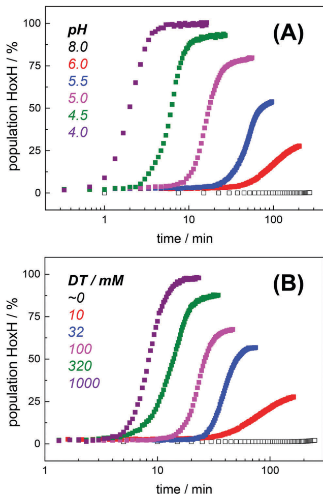
Fig. 4 Hox \rightarrow HoxH conversion in \text{HYDA1}^{\text{adt}} as a function of pH and dithionite concentration. (A) Increase of the HoxH population at a constant DT concentration of 10 mM and pH 6–4 in the aerosol. No HoxH is observed at pH 8 (open squares). (B) Increase of the HoxH population at a constant pH of 6 and varying DT concentration (10–1000 mM) in the aerosol. No HoxH is observed in the absence of DT (open squares, residual DT might still be present in the preparation). Each data point in (A) and (B) corresponds to a normalized IR spectrum for which the relative HoxH population (in %) was calculated from the respective sum of \text{CO}/\text{CN}^- peak areas.
